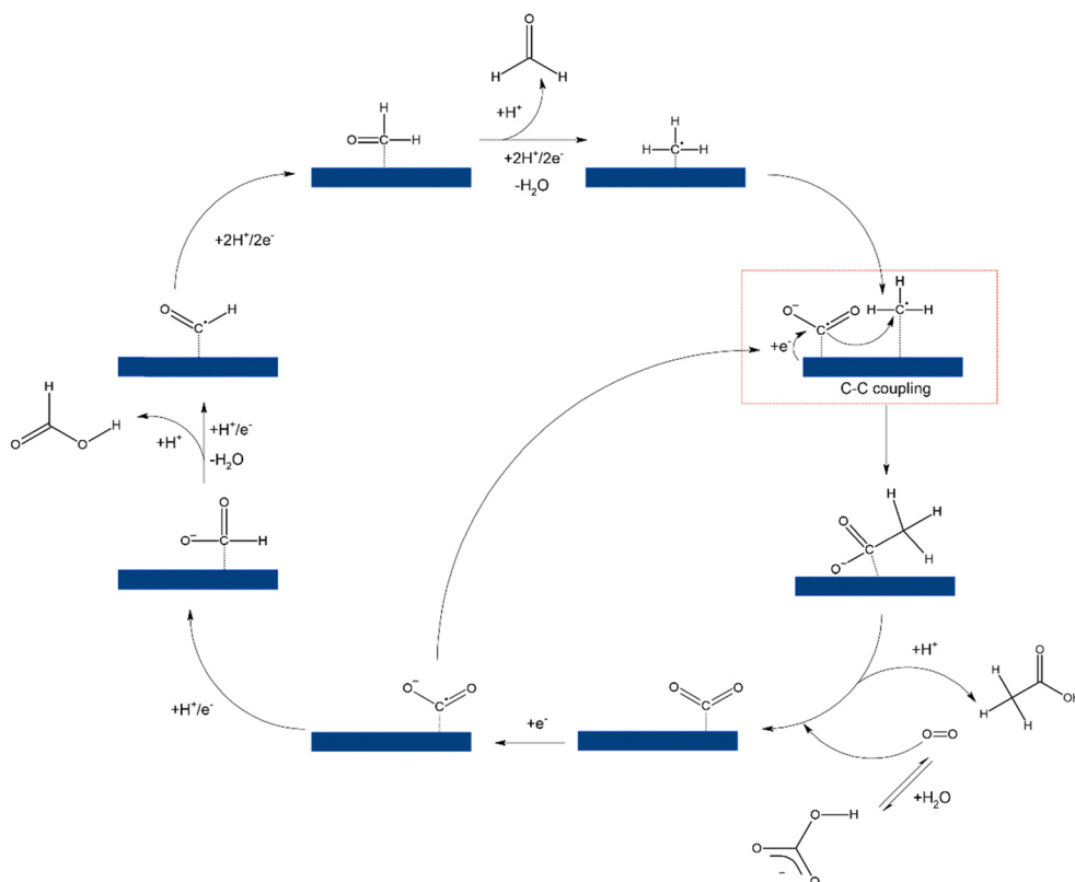
Scheme 1 Proposed reaction pathway of \text{CO}_2 to \text{HCOOH} , HCHO and \text{CH}_3\text{COOH} on AgPt NPR.
