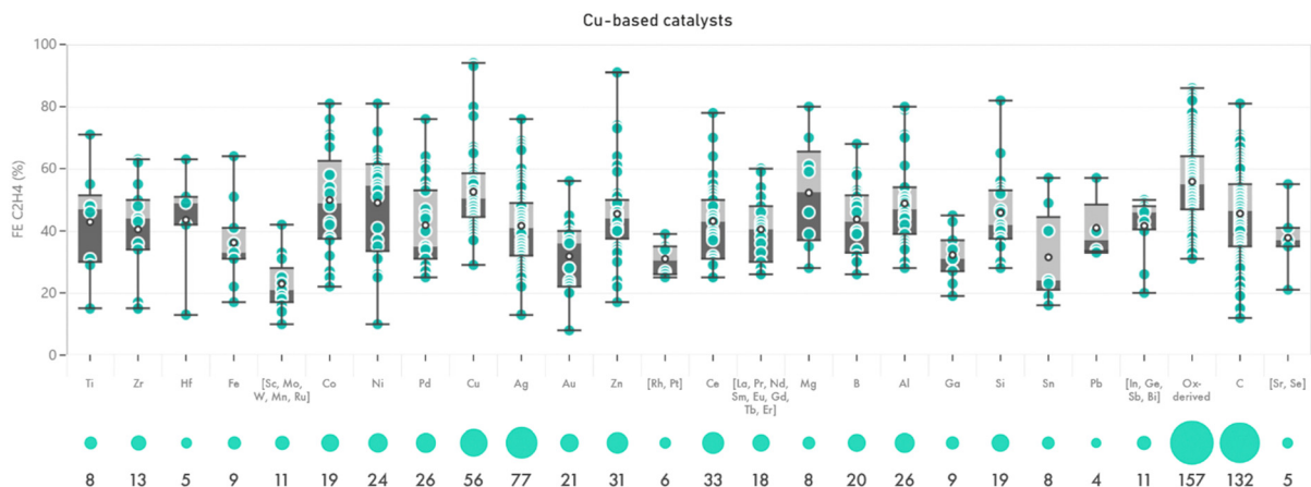
Fig. 1 High-level overview of the catalyst systems compiled in this work, depicting the maximum C 2 H 4 FE distribution for the catalyst systems as grouped based on their elemental composition, together with the number of sources identified for each of these categories.
