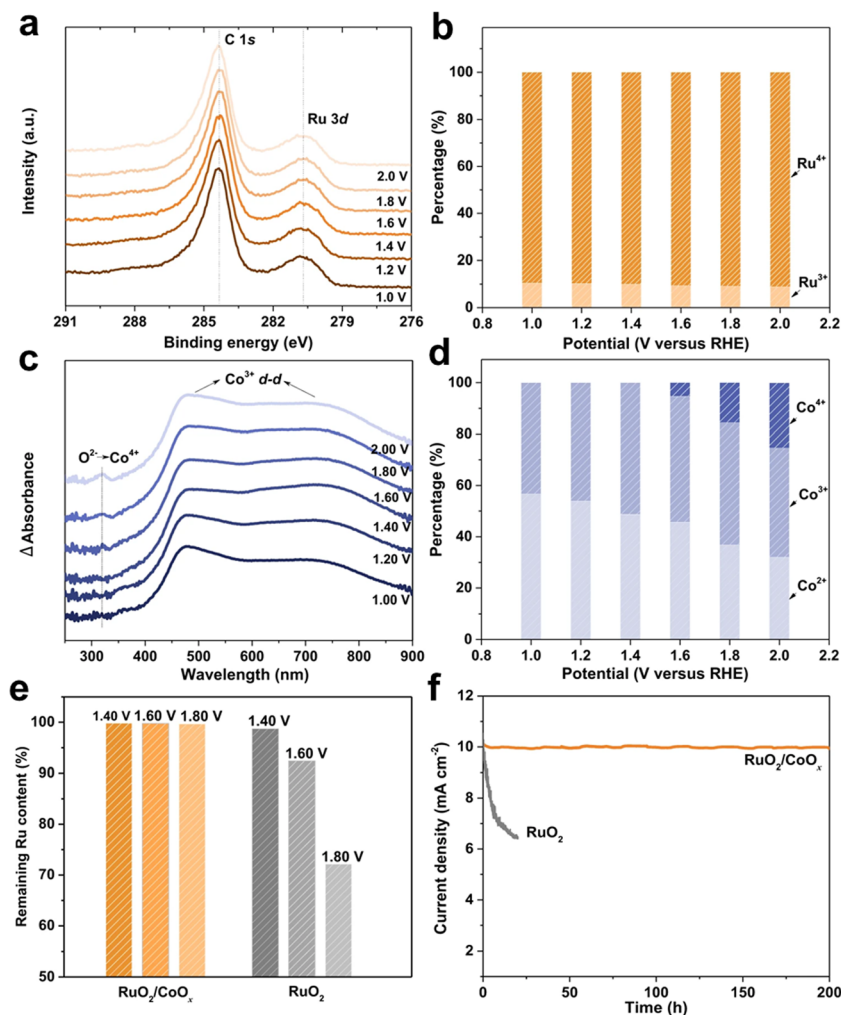
Fig. 7 Investigation on the in situ stability of an RuO 2 /CoO x hybrid catalyst during the OER. (a) and (b) In situ Ru 3d XPS spectra. (c) In situ UV-vis spectra. (d) Co 2+ , Co 3+ and Co 4+ content ratios in RuO 2 /CoO x under different applied potentials based on EPR analysis. (e) Retention ratios of Ru in RuO 2 /CoO x and RuO 2 after continuously testing at different potentials for 20 h. (f) Potentiostatic tests of RuO 2 /CoO x (at 1.47 V RHE ) and RuO 2 (at 1.59 V RHE ) for an initial current density of 10 mA cm -2 . Reprinted with permission from ref. 34 Copyright 2022, Springer Nature.
