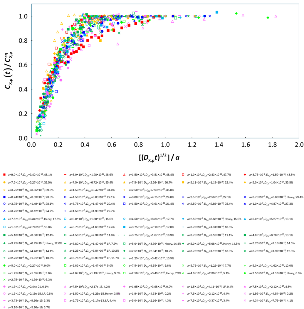
Fig. 6 Normalized kinetic sorption curves for data sets with <50% bulk depletion of the contaminant. For each data set, the legend gives the particle radius ( a (m)), the intraparticulate diffusion coefficient ( D_{X,p} ( m^2 s^{-1} )), and the % bulk depletion. Unless otherwise specified, the Langmuir isotherm is the best fit for the equilibrium data.
