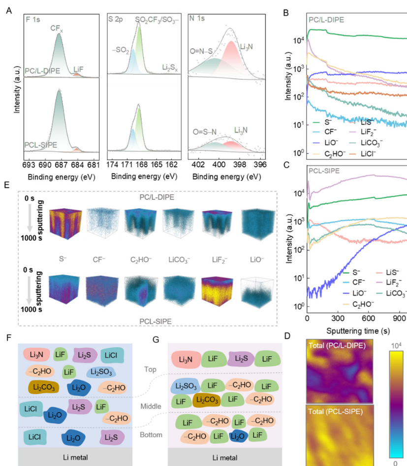
Fig. 5 Examination of SEI compositions of cycled Li metal recovered from Li|PC/L-DIPE|Li and Li|PCL-SIPE|Li cells. (A) F 1s, S 2p, N 1s ex situ XPS spectra. (B and C) Depth profiling of representative SEI components. (D) Comparative 2D rendered images of overall component distribution in the SEI layer. (E) Comparative 3D rendered images of representative sputtered secondary-ion fragments of SEI layers. (F and G) Schematic representation of the SEI compositions in the PC/L-DIPE and PCL-SIPE systems.
