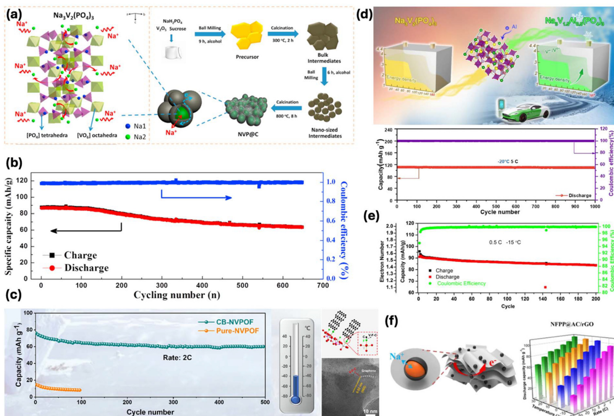
Fig. 10 (a) Schematic representation of \text{Na}^+ transport via hopping mechanism within the crystalline lattice, and synthesis route of the \text{NVP@C} nano-composite. (b) Extended cycling stability of \text{NVP@C} evaluated at -20^\circ\text{C} . 38 (c) Cycling performance of the pure NVPOF and CB-NVPOF at -40^\circ\text{C} . 143 (d) Long-term cycling stability of \text{Na}_3\text{V}_{1.5}\text{Al}_{0.5}(\text{PO}_4)_3 at a rate of 5. 145 (e) Cycling performance of NVCP at 0.5C and -15^\circ\text{C} in a three-electrode setup. 146 (f) Bar graph showing NFPP@AC/rGO discharge capacities across various rates and temperatures. 148
