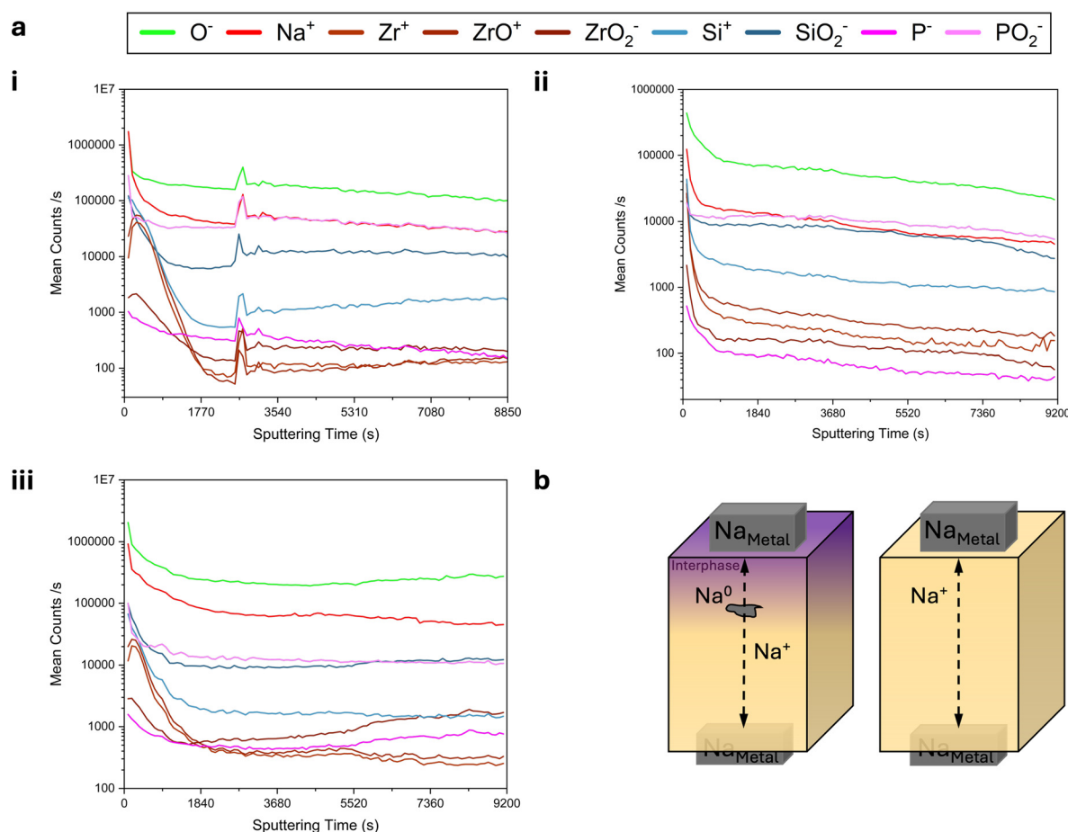
Fig. 4 Depth profiles of non-sodiated and sodiated regions. (a) Profiles of NASICON species and secondary phases with polarity chosen to maximise the yield. (i) A non-sodiated region, (ii) 0.04\text{ }\mu\text{A }\mu\text{m}^{-2} , and (iii) 0.1\text{ }\mu\text{A }\mu\text{m}^{-2} . (a)(i) Spike seen in the profile for the non-sodiated region is due to instrument artifact. (b) Schematic representation of the impact that the SEI has on sodium transport during cycling; dead sodium metal ( \text{Na}^0 ) nucleates inside the NASICON solid electrolyte due to reduced mobility along the grain boundaries.
