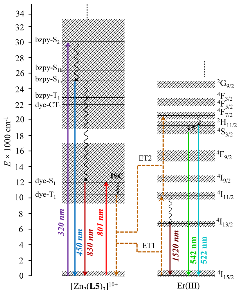
Fig. 6 Jablonski diagram established for [ZnErZn(L5) 3 ] 10+ , illustrating the mechanisms for inducing light downshifting and light UC through ligand-sensitized ETU. ET = intramolecular S → A energy transfer; ISC = intersystem crossing. The dye-centered triplet states are located according to ref. 62.
