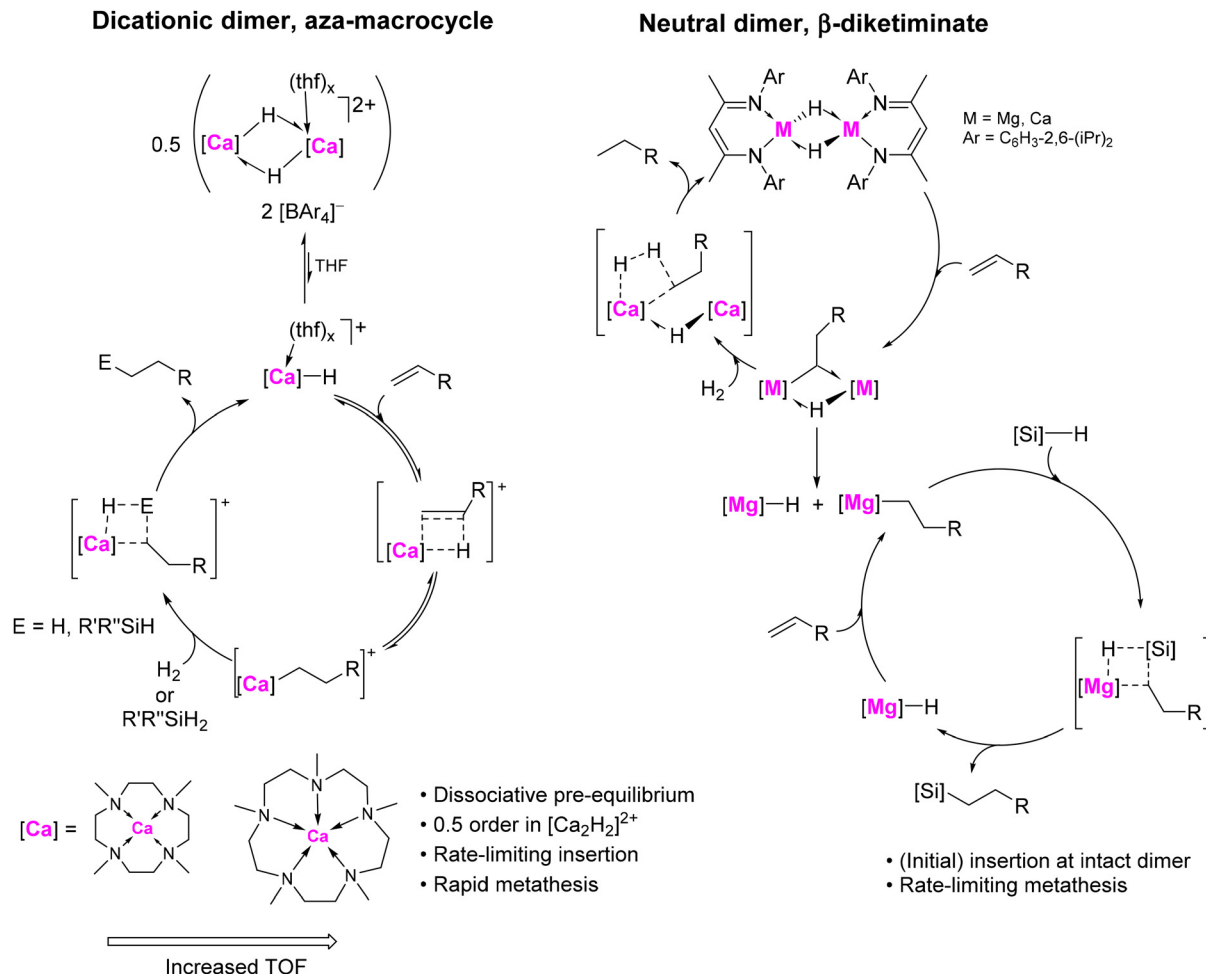
Scheme 20 Contrast in proposed mechanisms for olefin hydrogenation and hydrosilylation mediated by \text{Me}_4\text{TACD}/\text{Me}_5\text{PACD} -calcium and \text{BDI}^{\text{dipp}} -calcium/magnesium catalysts.
