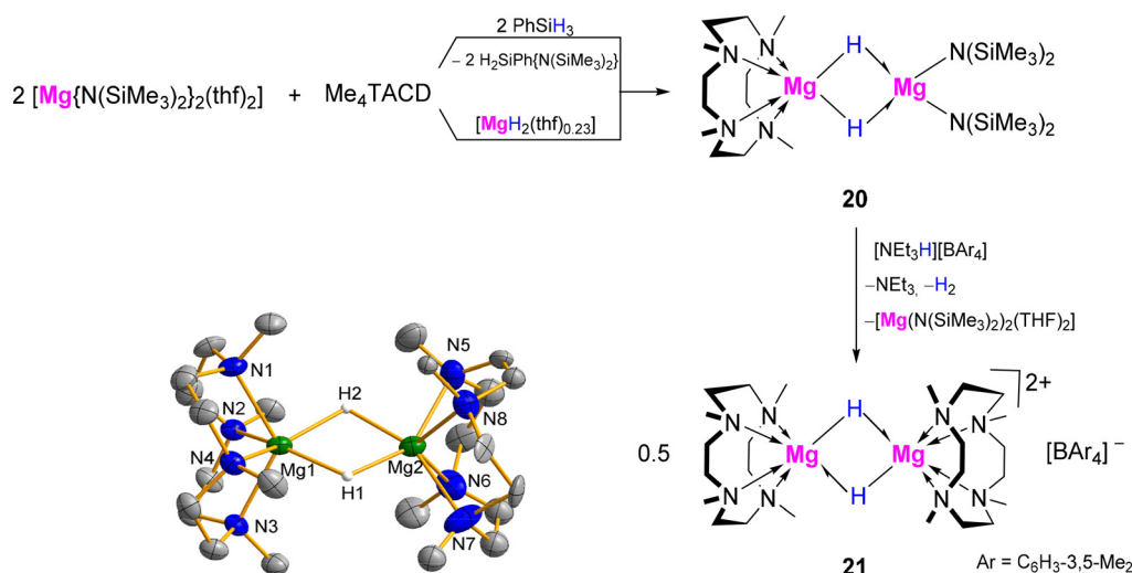
Scheme 6 Me 4 TACD-supported magnesium hydrides 20 and 21 and the molecular structure of the dicationic part of 21 . Ar = C 6 H 3 -3,5-Me 2 .
