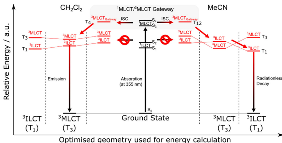
Fig. 2 Relative energies of excited states and transitions for 8 in \text{CH}_2\text{Cl}_2 and \text{MeCN} . Reprinted with permission from ref. 104 Copyright © 2021, American Chemical Society.
