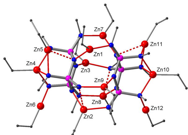
Fig. 2 Crystal structure of the dimeric complex 5 . Zn, red; N, blue; P, purple; C, grey. Hydrogen atoms are omitted for clarity.
