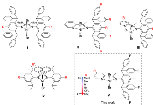
Chart 1 Selected examples of Ni(II) ethylene polymerisation precatalyst (I–IV), including this work (V), and the sites on their ligand framework (R) used to study electronic effects.
