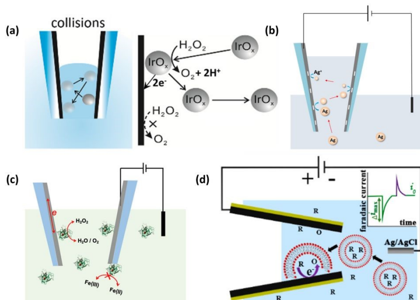
Fig. 5 (a) Experimental setup for monitoring collisions of a NP with a carbon nanopipette. Reproduced from Ref [28], with permission from American Chemical Society, copyright 2017. (b) Electrochemical collision and oxidation of single AgNPs inside carbon nanopipettes. Reproduced from Ref [29], with permission from American Chemical Society, copyright 2021. (c) Electrochemical collision of single horseradish peroxidase enzyme inside carbon nanopipette via catalytic amplification. Reproduced from Ref [30], with permission from American Chemical Society, copyright 2022. (d) Resistive-pulse experiments involving translocation of liposomes through carbon nanopipettes. Reproduced from Ref [31], with permission from American Chemical Society, copyright 2019.
