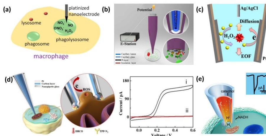
Fig. 6 (a) ROS/RNS analysis in living cells. Reproduced from Ref [84], with permission from American Chemical Society, copyright 2019. (b) Schematic of the nanokit used for the single-cell electrochemical analysis. Reproduced from Ref [85], with permission from National Academy of Sciences, copyright 2016. (c) The electroosmotic flow inside the conductive nanopipettes to help enrich the analytes of interests to allow the sensitive detection of low-abundance proteins. Reproduced from Ref [86], with permission from American Chemical Society, copyright 2022. (d) Electrochemical setup for the capture and dynamic measurement of ROS released from one mitochondrion in a living MCF-7 cell. Voltammograms of FcMeOH with the nanopipette before (i) and after (ii) capturing one mitochondrion inside the living cell. Reproduced from Ref [87], with permission from Wiley, copyright 2023. (e) The asymmetric nanopore electrode for single-cell probing. Reproduced from Ref [78], with permission from American Chemical Society, copyright 2018.
