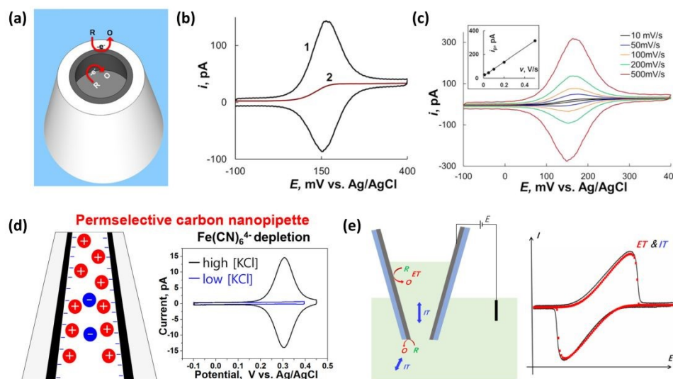
Fig. 4 Thin-layer electrochemistry inside the conductive nanopipettes. (a) Schematic representation of the thin-layer electrochemistry inside the cavity and at the carbon ring at the pipette orifice. (b) Cyclic voltammograms of 1 mM ferrocenemethanol in 0.2 M KCl solution obtained using an \sim 100 nm radius CNP at different potential sweep rates, v=10 mV/s (1) and 200 mV/s (2). (c) A family of curves obtained for the range of v from 10 to 500 mV/s. Panel a, b and c are reproduced from Ref [21], with permission from American Chemical Society, copyright 2014. (d) The electric double layer effect on the resulting CV responses, with enriched redox cations and depleted redox anions inside the nanopipettes. Reproduced from Ref [53], with permission from American Chemical Society, copyright 2019. (e) The coupled electron transfer processes and ionic transport processes inside the carbon nanopipettes, leading to the sloped thin-layer electrochemical behaviours in the resulting CV responses. Reproduced from Ref [16], with permission from Royal Society of Chemistry, copyright 2021.
