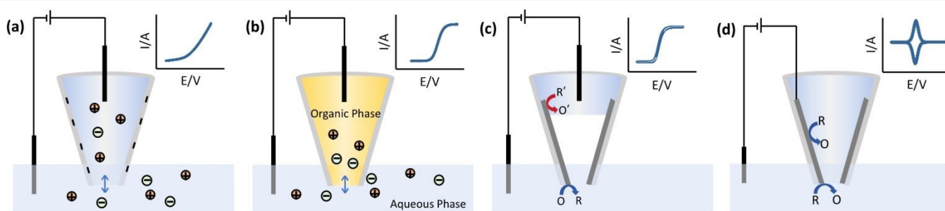
Fig. 2 Schematic representation of (a) Ion current rectification (ICR), (b) Electrochemistry through liquid/liquid interface, (c) Bipolar electrochemistry and (d) Thin-layer electrochemistry in the nanopipettes.
