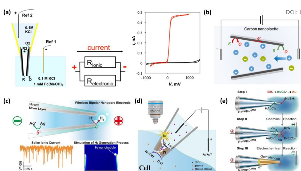
Fig. 3 The bipolar electrochemistry inside the conductive nanopipettes. (a) The experimental setup of the bipolar electrochemistry at the conductive nanopipettes. The current would include both ionic current through the pipette and the electronic current through the conductive layer, so that Z-shaped CV response would be resulted once the ionic transport is prohibited. Reproduced from Ref [11], with permission from American Chemical Society, copyright 2014. (b) The redox mediator would affect the floating potential of the carbon layer, and the resulting ionic current rectification through the carbon nanopipettes. Reproduced from Ref [46], with permission from American Chemical Society, copyright 2017. (c) The silver coated nanopipette could serve as wireless bipolar nanopore electrode to sensitively detect various analytes of interests such as \text{H}_2 and \text{Ag}^+ . Reproduced from Ref [17], with permission from American Chemical Society, copyright 2017. (d) The deposition of Pt inside the nanopipette would allow the coupled electrochemical reaction inside the cells with the electrochemiluminescence at the other end of the Pt layer, allowing the detection of intracellular hydrogen peroxide or glucose as well as the sphingomyelinase activity. Reproduced from Ref [18], with permission from Wiley, copyright 2020. (e) A closed bipolar setup in glass nanopipettes fabricated with a simple chemical-electrochemical method. Reproduced from Ref [20], with permission from Wiley, copyright 2017.
