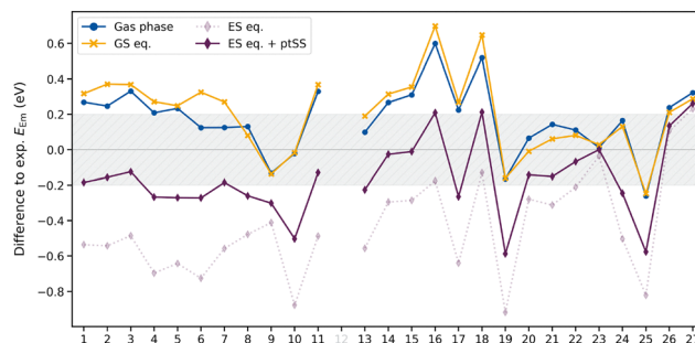
Fig. 5 Emission energies computed using DFT/MRCI with the R2018 Hamiltonian and short settings at the ROKS S_1 geometries. The DFT/MRCI anchor configuration (BHLYP/def2-SVP(P)) was computed in gas phase (blue), using ground state equilibrium solvation conditions with the COSMO implicit solvation model (denoted "GS eq.", orange) or the S_1 excited state reaction field without (denoted "ES eq.", light purple) and with ptSS-PCM correction ("ES eq. + ptSS", purple) obtained from ROKS-OT-LC- \omega PBE/def2-SVP+PCM. An uncertainty of 0.20 eV for the experimental references is assumed and represented as grey shading.
