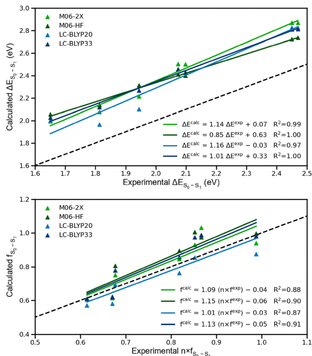
Fig. 6 S_1 vertical excitation energies (top) and oscillator strengths (bottom) of different TD-DFT methods plotted against their respective \lambda_{max} and peak surface derived experimental counterparts. The dashed lines represent perfect coincidence of the theoretically and experimentally obtained values.
