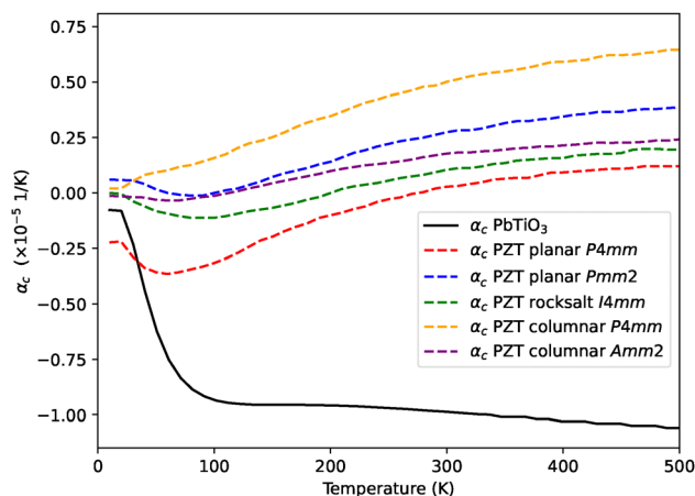
Fig. 3 Thermal expansion coefficients in the c direction, \alpha_c ( \text{K}^{-1} ), calculated with quasi-harmonic approximation in a temperature range of 10 to 500 K. Data for \text{PbTiO}_3 from ref. 34.
