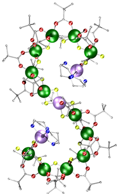
Fig. 1 Crystal structure of [\text{Ni}(\text{cyclen})]_2\text{Cr}_{12}\text{NiF}_{18}(\text{O}_2\text{C}^t\text{Bu})_{24} 1 (where cyclen = 1,4,7,10-tetraazacyclododecane). Colours: Cr, green; Ni, purple; F, yellow; O, red; N, blue; C, grey. Hydrogen atoms are omitted for clarity.
