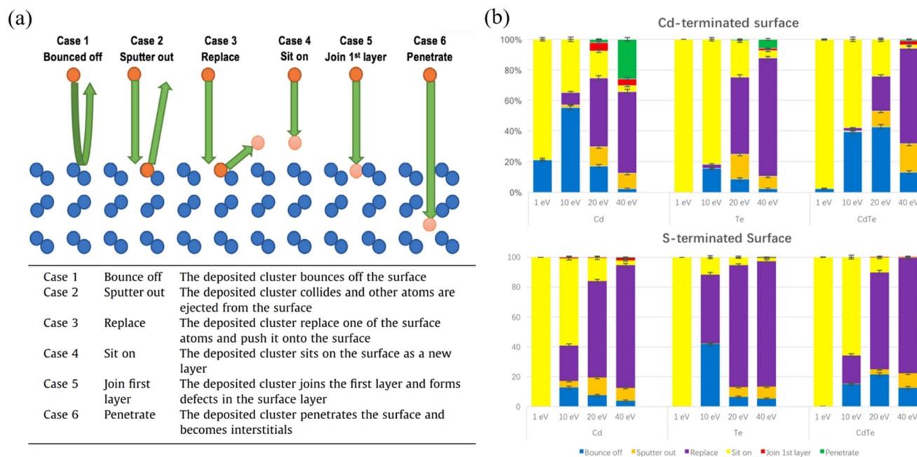
Fig. 5 (a) The illustration graph for the 6 cases of the final states after impact. (b) Energetic impact results of small Cd x Te y (x, y = 0, 1) clusters on wurtzite (111) Cd-terminated and S-terminated CdS surfaces (copyright from Elsevier, Nuclear Instruments and Methods in Physics Research B). 55
