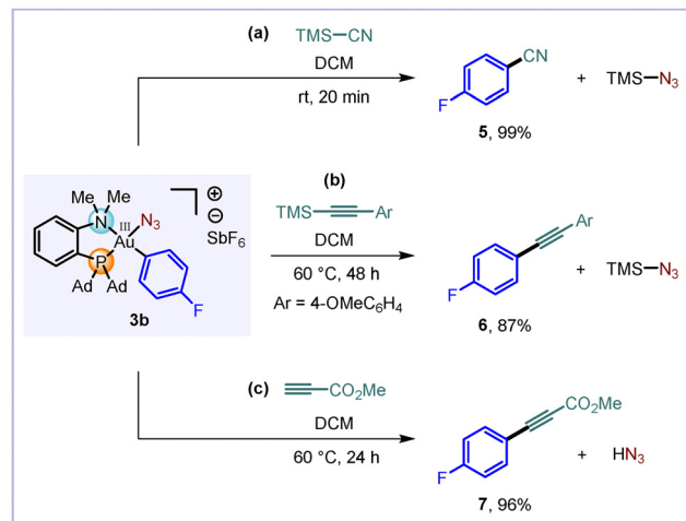
Scheme 4 Reactivity of (P ^ N) aryl Au(III)-azide complex towards ligand exchange and reductive elimination processes. a (a) Reaction with TMS-CN. Conditions: 0.20 mmol 3b , 1.0 mmol TMS-CN, DCM (0.1 M), rt, 20 min. (b) Reaction with TMS-alkyne. Conditions: 0.20 mmol 3b , 1.0 mmol TMS-alkyne, DCM (0.1 M), 60 °C, 48 h. (c) Reaction with terminal alkyne. Conditions: 0.20 mmol 3b , 1.0 mmol methyl propiolate, DCM (0.1 M), 60 °C, 24 h. a Isolated yields.
