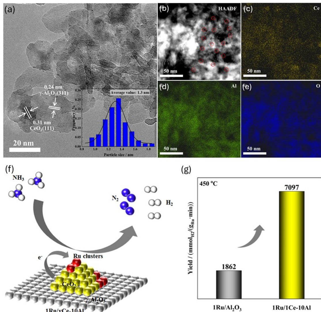
Fig. 17 (a) HRTEM image and particle size distribution (inset); (b) HAADF image (the Ru clusters are marked with red circles); (c)–(e) EDS elemental mapping images including Ce, Al, and O of used 1\text{Ru}/1\text{Ce}-10\text{Al} catalyst. (f) Graphical representations of Ru clusters are dispersed on Ce–Al support and enhanced hydrogen yield. (Reproduced from ref. 104. Copyright (2023), with permission from Elsevier).
