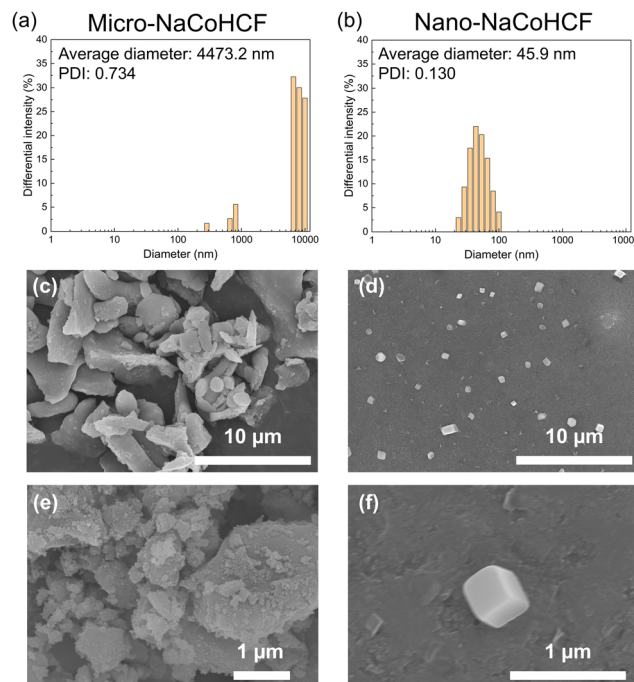
Fig. 2 (a) and (b) Intensity-weighted size distributions of the micro-NaCoHCF and nano-NaCoHCF particles measured by dynamic light scattering (DLS). The average diameters and polydispersity index (PDI) were calculated using the cumulant method. (c)–(f) SEM images of the synthesized NaCoHCF particles. (c) Micro-NaCoHCF with low magnification, (d) nano-NaCoHCF with low magnification, (e) micro-NaCoHCF with high magnification, and (f) nano-NaCoHCF with high magnification.
