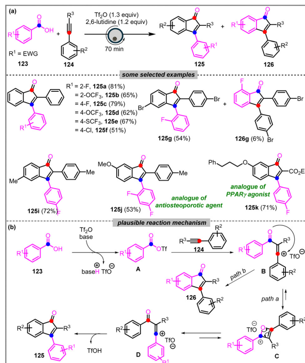
Scheme 23 (a) Solvent-free mechanochemical indanone synthesis via an unprecedented aryl migration under ball milling. (b) Plausible reaction mechanism for indanone synthesis.
