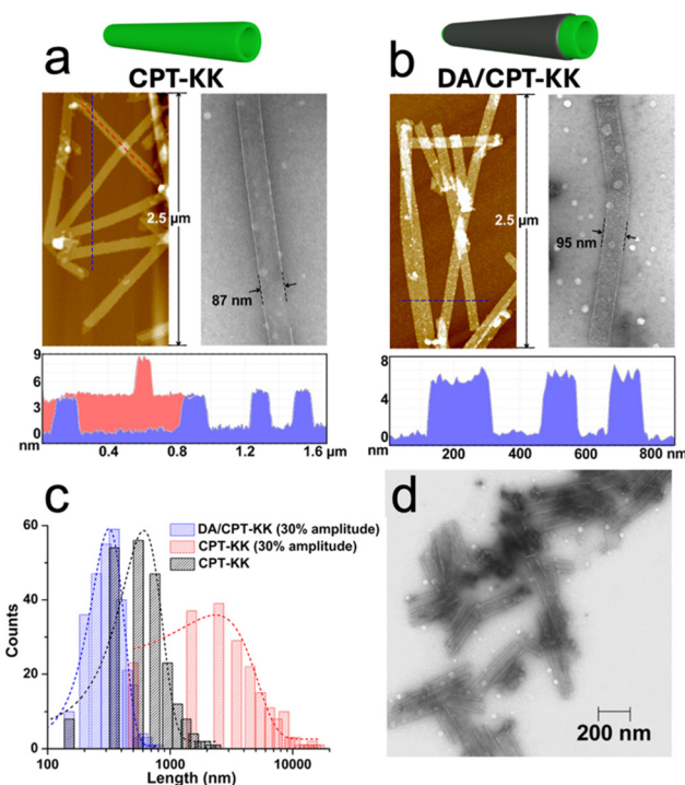
Fig. 2 AFM height profiles and TEM images of (a) CPT-KK and (b) DA/CPT-KK (5 : 1, n/n) in PBS. After incubation in PBS (10 mM with respect to CPT-KK ) for 24 h, samples of CPT-KK and DA/CPT-KK were diluted to 1 mM (PBS) prior to AFM and TEM imaging. After coating CPT-KK nanotubes with PDA, the wall thickness increased from 2 nm for CPT-KK to ~3.3 nm for DA/CPT-KK . (c) Histograms of length distributions, measured from TEM images, of CPT-KK with and without sonication (37.5 W for 1 min) and DA/CPT-KK (5 : 1, n/n, sonicated). (d) TEM image of DA/CPT-KK after sonication (37.5 W, 1 min).
