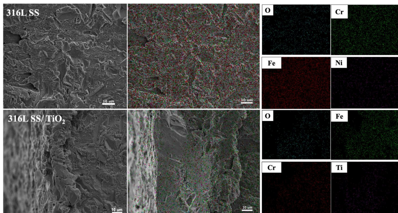
Fig. 1 SEM micrographs of 316L SS and 316L SS/TiO 2 surfaces. SEM micrographs reveal a rough surface because of the sandblasting. In addition to the presence of characteristic elements of SS, mapping analysis confirms the presence of Ti.
