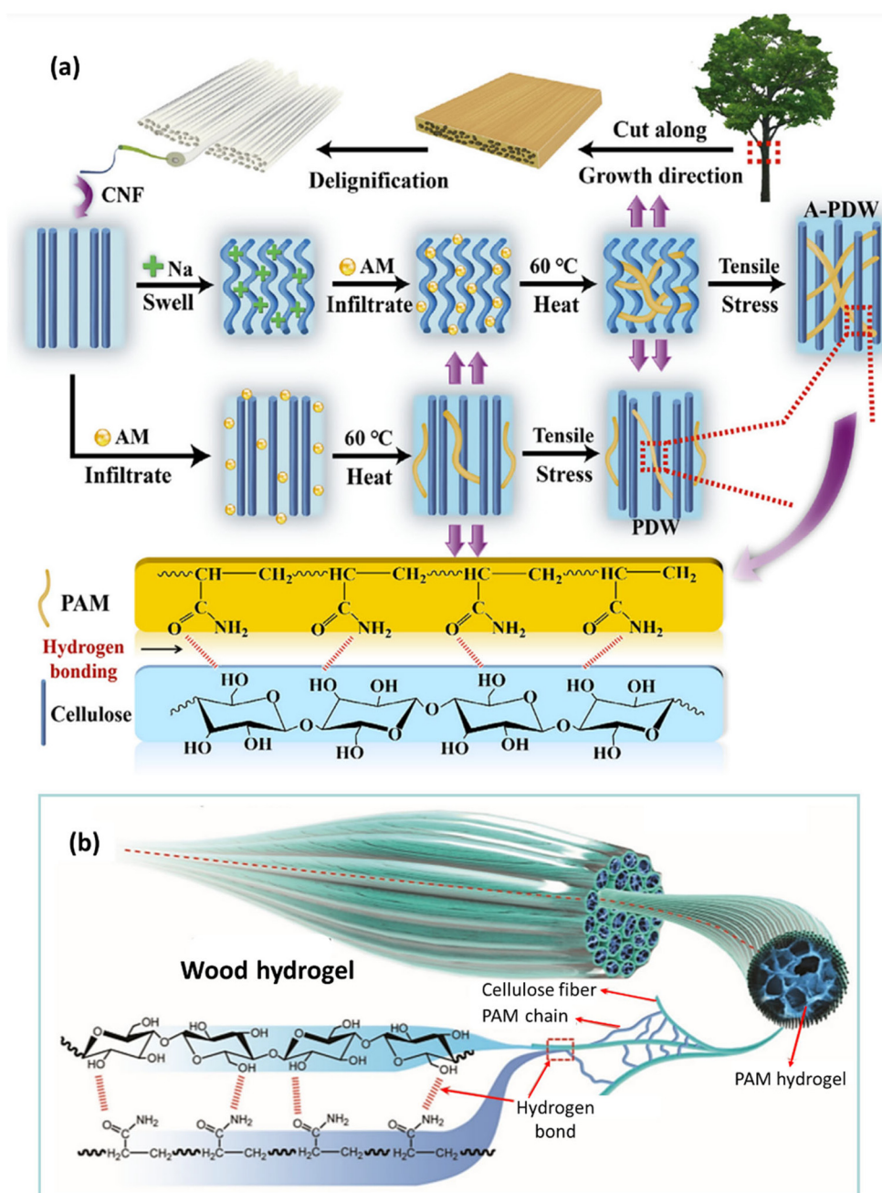
Fig. 17 Physical coating of plant-based scaffolds. Schematic illustration of wood modification with (a) a PAM polymer network using in situ chemical free-radical polymerization. (Reprinted from ref. 64 with permission from Elsevier B.V. Copyright 2020.) (b) Muscle-inspired wood hydrogel prepared through free-radical polymerization, showing hydrogen bonds and covalent cross-linking between PAM chains and CNFs. (Reproduced from ref. 152 with permission from WILEY-VCH Verlag GmbH & Co. Copyright 2018.)
