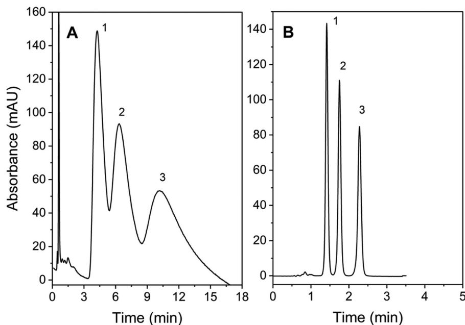
Fig. 4 Chromatograms illustrating the separation of model compounds in columns with p -PDA-derived phases containing (A) 13 rings per nm 2 and (B) 4 rings per nm 2 on 5 µm-Kinetex® core-shell silica particles (columns dimensions: 50 mm length, 2.1 mm i.d.). A mobile phase of 50/50 acetonitrile/water was used at a flow rate of 0.2 mL min -1 ; UV detection was performed at 210 nm. Compounds: (1) toluene, (2) ethylbenzene, and (3) propylbenzene (100 µg mL -1 each, 1 µL injection).
