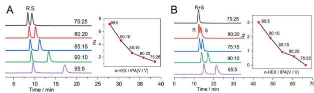
Fig. 8 Enantioseparations of (A) 1-phenylethanol on column A and (B) ethyl mandelate on column B using different ratios of n -HEX/IPA as mobile phases (column temperature: 25 °C; flow rate: 0.1 mL min -1 ).
