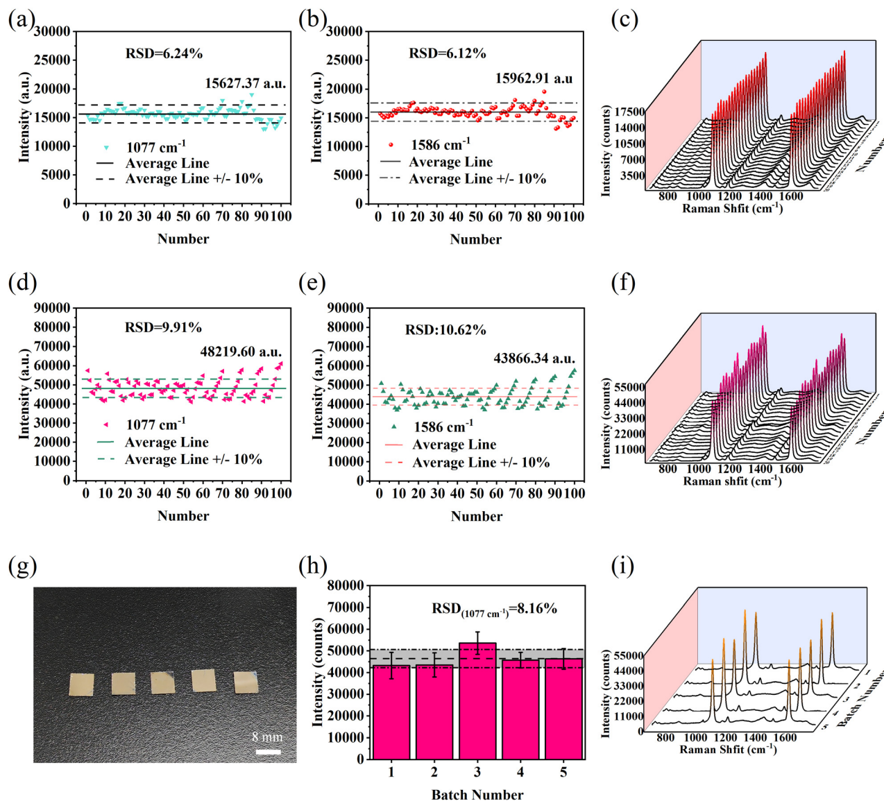
Fig. 4 (a) Raman intensity of characteristic peaks at 1077 cm -1 and (b) 1586 cm -1 for 4-MBA (10 -4 M) on Au nanosphere array. (c) Raman spectra from 20 random spots on Au nanosphere array. (d) Raman intensity of characteristic peaks at 1077 cm -1 and (e) 1586 cm -1 for 4-MBA (10 -4 M) on Au nanostar array. (f) Raman spectra from 20 random points on Au nanostar array. (g) Photograph of five different batches of Au nanostar arrays on Si wafers with each size of 0.8 × 0.8 cm 2 . (h) Raman intensity at peak 1077 cm -1 and (i) Raman spectra of 4-MBA (10 -4 M) obtained from five different batches of Au nanostar arrays.
