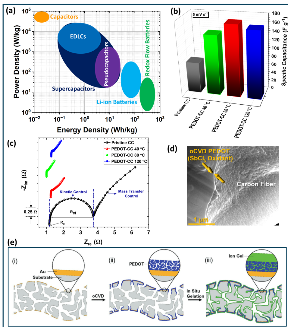
Fig. 13 Utilization of PEDOT conducting polymer coatings in supercapacitors. (a) Ragone plot illustrating the relative positions of EDLC and pseudocapacitors, showing how supercapacitors bridge the gap between batteries and traditional capacitors in terms of energy and power density. (b) Specific capacitance values for carbon cloth (CC) and oCVD PEDOT-coated carbon cloth (PEDOT-CC) electrodes. The oCVD PEDOT thin films fabricated at different deposition temperatures. 10 (c) Nyquist plots for pristine carbon cloth and PEDOT-coated carbon cloths fabricated at different deposition temperatures. 10 (d) Magnified SEM image showing an individual carbon fiber with a highly conformal oCVD PEDOT coating. 10 (e) Schematic illustrations of the intermediate and final configurations of a vapor-printed solid-state supercapacitor, where gray for porous substrate, gold for current collector, blue for PEDOT, and green for ion gel electrolyte. 272 (b)–(d) Reproduced with permission. 10 Copyright 2024, Wiley. (e) Reproduced with permission. 272 Copyright 2017, Wiley.
