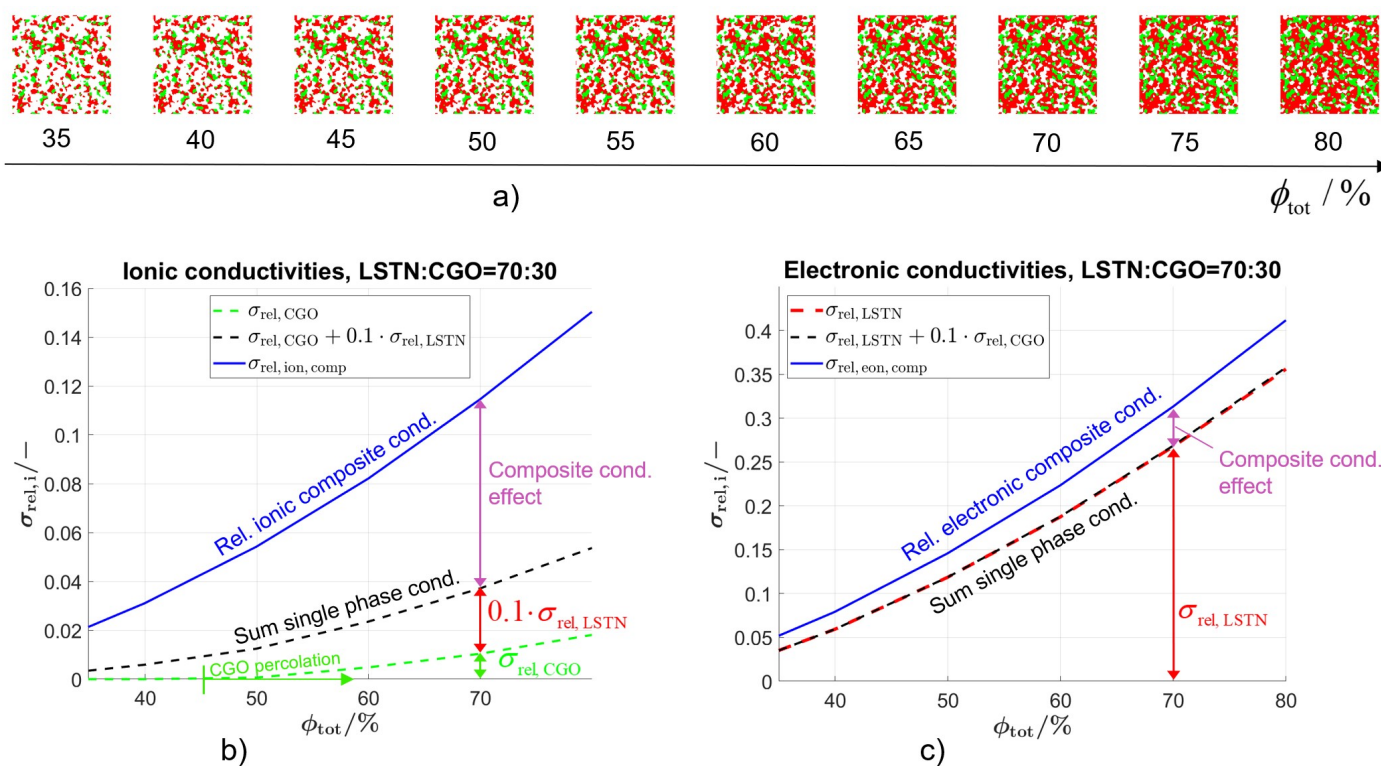
Fig. 7 a) Virtual structures of ceramic anodes with constant solid-phase composition (i.e., 70 % LSTN and 30 % CGO), but with increasing total solid volume fractions ( \phi_{\text{tot}} ) from left to right (and with decreasing porosity, respectively). b) Illustration of the three contributions, which constitute the total ionic composite conductivity in MIEC anodes with varying porosity. These contributions are the effective ionic conductivities of isolated LSTN (red) and isolated CGO-phases (green). In addition, there is a specific composite contribution (magenta), which originates from the fact that obstacles to ionic transport (e.g., bottlenecks and dead ends) in one phase can be by-passed by ionic transport through the other phase. Note that the contribution from LSTN must be weighted by 0.1, because its intrinsic ionic conductivity is 10 times smaller compared to CGO. c) Vice versa for the electronic composite conductivity: In this case, the isolated CGO-part (green) has only an inferior contribution to the sum of single-phase conduction (black) due to a combined effect from low intrinsic electronic conductivity and low volume fraction of CGO in these anode microstructures. Hence, single-phase conduction in the LSTN-phase (red) represents the main contribution to the total electronic conduction. Nevertheless, there is also a considerable contribution associated with the composite conductivity effect (magenta). However, in these anodes the composite contribution is much larger for ionic than for electronic conduction, as illustrated by the different magnitudes of magenta contributions in b) and c).
