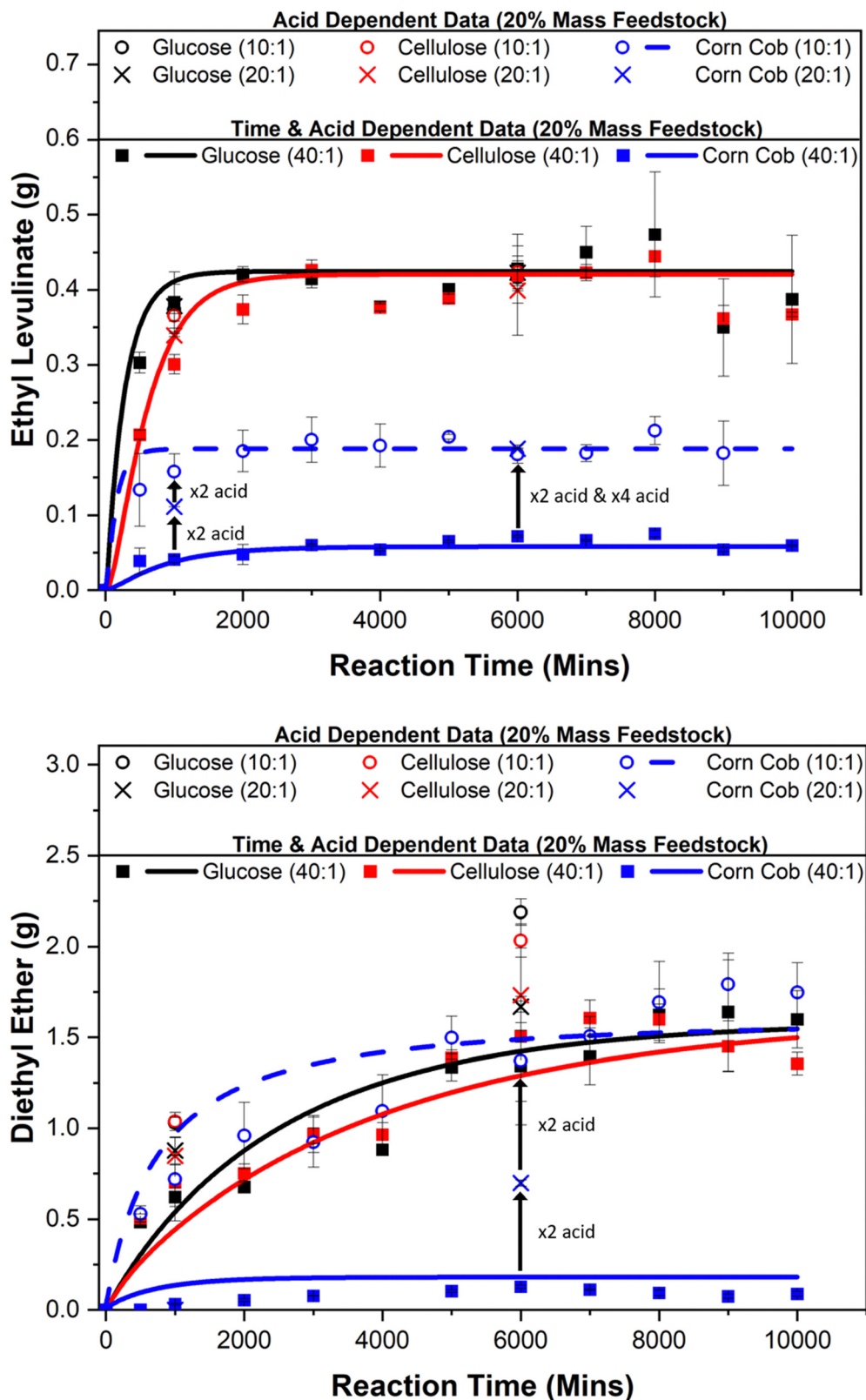
Fig. 5 Ethyl levulinat (g) and diethyl ether (g) produced from the sulphuric acid-catalysed ethanolysis of glucose, cellulose, and corn cob (5, 10, and 20 mass percent) for three different feedstock-to-acid ratios (10 : 1, 20 : 1, and 40 : 1) at 150 °C. Full time-dependent data sets are produced for a feedstock-to-acid ratio of 40. An additional time-dependent data set was produced for corn cob only at a feedstock-to-acid ratio of 10 : 1. At 1000 and 6000 minutes, reactions are performed varying the feedstock-to-acid ratio (10 : 1, 20 : 1, and 40 : 1) to determine the acid dependence of the process in both the kinetic and steady-state phases. The square, cross, and circle data points represent experimental data, and the lines represent the chemical kinetic model.
