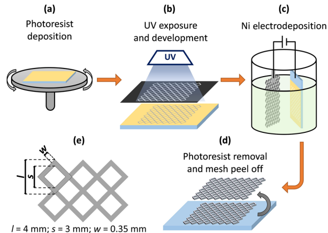
Fig. 1 Sketch of the Ni mesh fabrication process.
