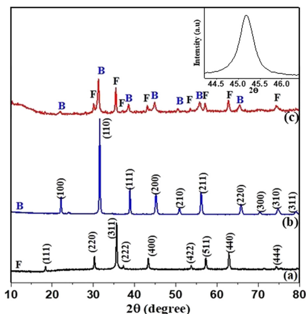
Fig. 3 XRD pattern of (a) NCMF, (b) BT, (c) NCMF@BT nano powders, and the inset graph shows the XRD of NCMF@BT at 45°.
