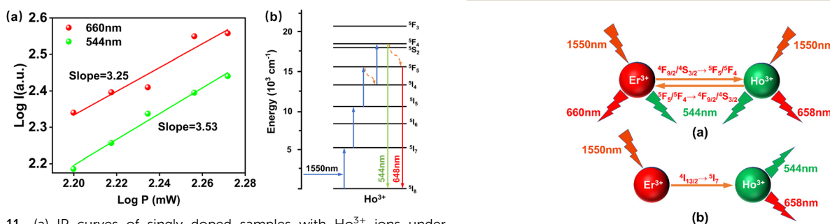
Fig. 13 (a) Schematic diagram of the reverse energy transfer of \text{Er}^{3+} – \text{Ho}^{3+} ions. (b) Schematic diagram of the energy transfer of \text{Er}^{3+} – \text{Ho}^{3+} ions.
