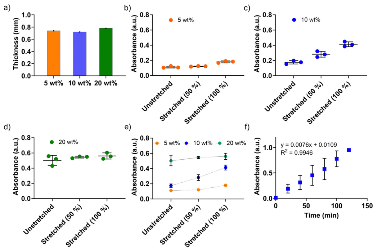
Fig. 5 (a) Thickness of P(St- stat - n BA)/FeSiNP films, (b)–(d) peroxidase enzyme-mimicking nanozyme activity of P(St- stat - n BA)/FeSiNP (5 wt%, 10 wt%, and 20 wt%, respectively) films under unstretched and stretched conditions at different stretching lengths, (e) combined peroxidase enzyme-mimicking nanozyme activity, (f) catalytic activity of P(St- stat - n BA)/10 wt% FeSiNP films over a 2 h reaction period.
