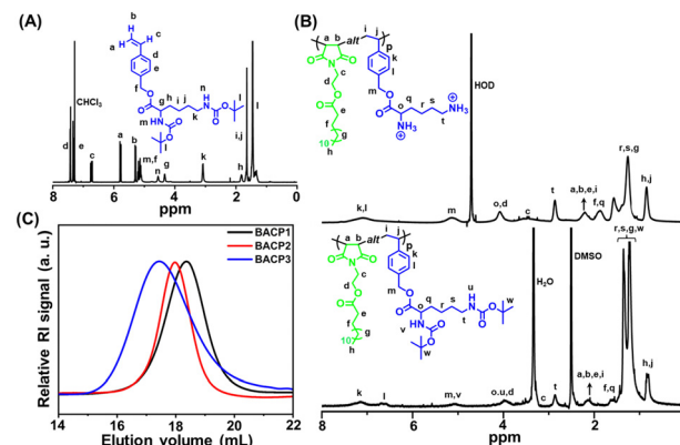
Fig. 1 (A) ^1\text{H} NMR spectrum of M2 . (B) ^1\text{H} NMR spectra of the protected polymer ( BACP3 ) in \text{DMSO}-d_6 and deprotected polymer ( ACPy ) in \text{D}_2\text{O} . (C) SEC RI traces of BACP1 – BACP3 in DMF.
