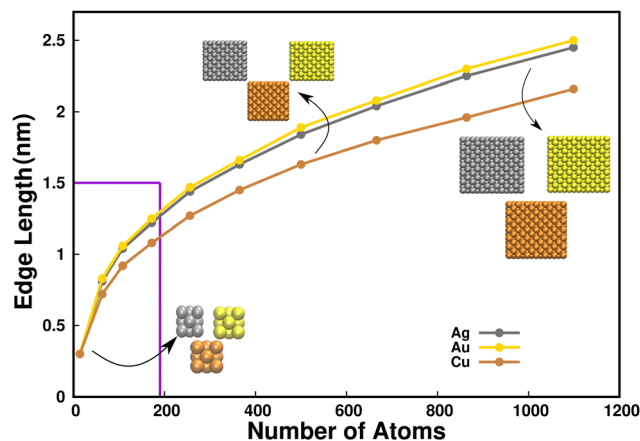
Fig. 1 The size ( N ) to edge length dimension comparison of cubic representative geometries corresponding to Cu, Ag and Au MNCs. The structures for N = 14500 , and 1099 can be identified in the inset. It can also be identified here that structures with N < 200 define an ultrasmall NC (edge length < 1.5 nm).
