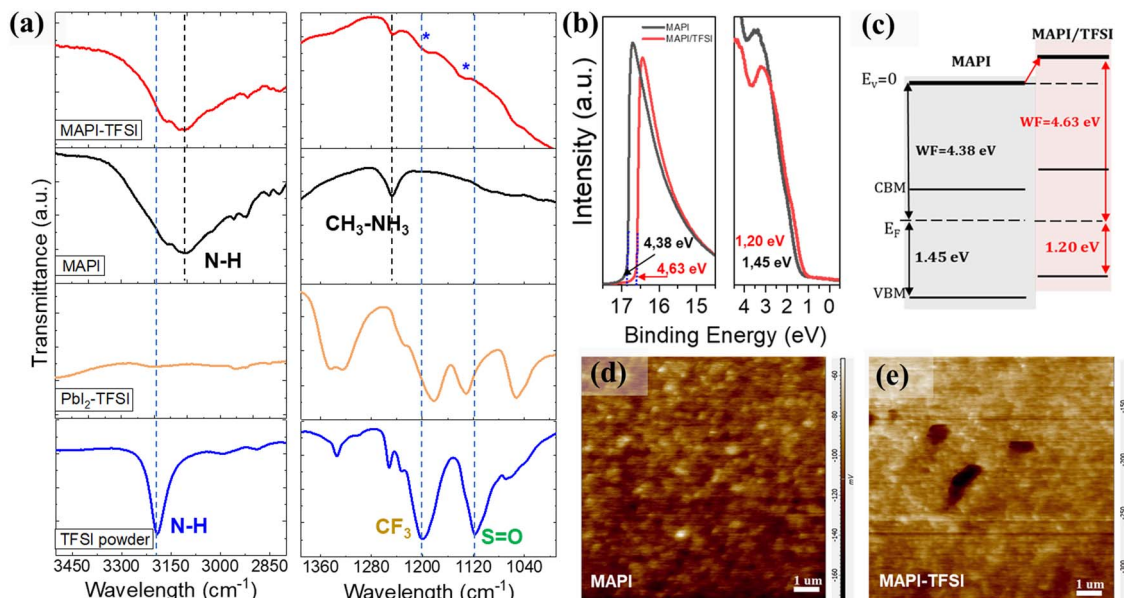
Fig. 4 FTIR spectra of the TFSI powder, PbI 2 -TFSI mixture, MAPI film and MAPI/TFSI film in a comparative presentation (a). UPS spectra (b), schematic diagram of the relative energy level positions (c), and Kelvin probe AFM images (d and e) of FTO/TiO 2 /MAPI and FTO/TiO 2 /MAPI/TFSI films of the corresponding devices.
