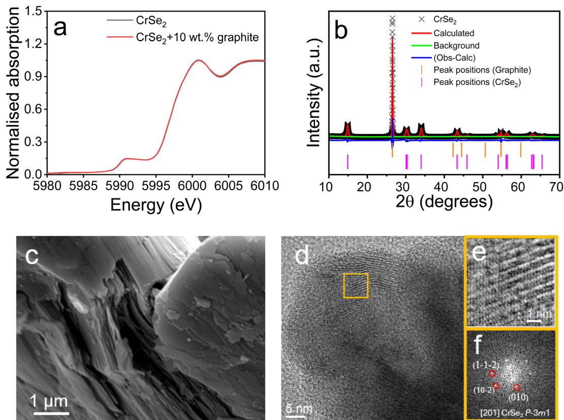
Fig. 2 (a) Cr K-edge XANES profile of pure \text{CrSe}_2 (black) and \text{CrSe}_2 with 10 wt% of graphite (red). (b) LeBail refinement of the experimental PXRD profile ( \text{CuK}_\alpha ) for a \text{CrSe}_2 with 10 wt% of graphite against relevant structure models for \text{CrSe}_2 and graphite. Experimental data are shown as black crosses; the calculated profile is shown by a solid red line. The difference between the calculated and experimental data is shown as a blue profile. Magenta and orange vertical bars represent the Bragg positions of the \text{CrSe}_2 and graphite phases. (c) SEM image of \text{CrSe}_2 with 10 wt% of graphite. (d) HRTEM image of \text{CrSe}_2 with 10 wt% of graphite. (e) HRTEM magnified detail of the yellow squared region in (d) showing the \text{CrSe}_2 crystalline structure. (f) Power spectra (Fourier Transform) applied to (e), with the corresponding crystal structure indexing.
