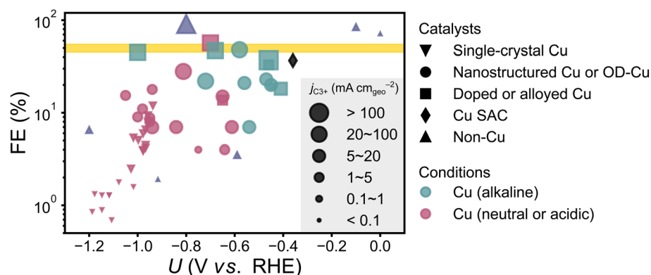
Fig. 10 A summary on catalytic performance of direct electrochemical CO 2 /CO-to-C 3+ conversion using different types of catalysts (including single-crystal Cu, nanostructured Cu or OD-Cu, doped or alloyed Cu with foreign element regulation, Cu SAC, and Mo- or Ni-based non-Cu catalysts). The first three types of catalysts are further divided into two groups to reveal the influence of electrolyte pH; cyan for the alkaline conditions where KOH electrolytes are adopted, and red for the neutral or acidic conditions where bicarbonates, halides, or other oxyanions are adopted. The size of markers indicates the magnitude of partial current density of C 3+ formation. Data for plotting are tabulated in Table S1.†
