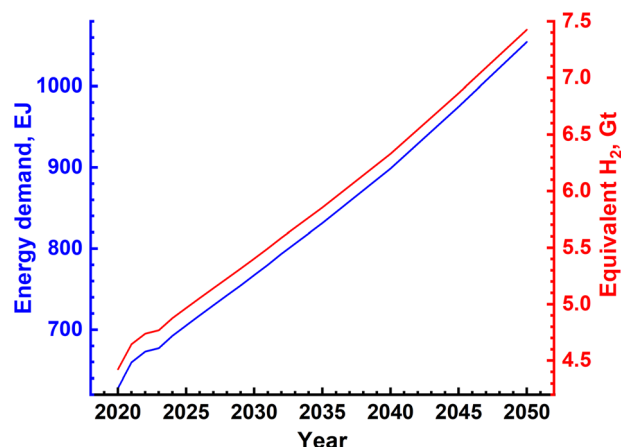
Fig. 7 Energy demand till the year 2050 has been forecasted by the US Energy Information Agency's Energy outlook report of 2023 and is shown here together with the equivalent amount of \text{H}_2 gas required to generate the yearly energy demand, assuming that complete energy requirement is met by \text{H}_2 . To convert the energy demand into equivalent \text{H}_2 amount, the higher heating value has been used, which gives the lower limit of gas requirement. The actual requirement will be higher than the value shown here.
