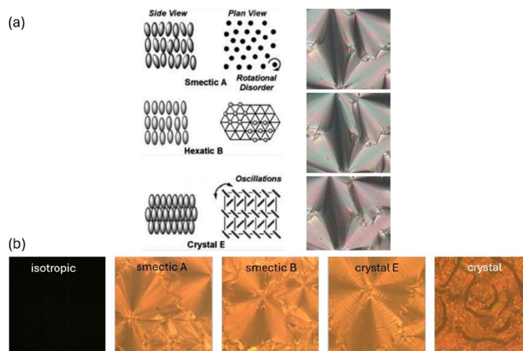
Fig. 3 (a) Structures of the liquid crystal phases investigated. Staring from elevated temperatures the fluid SmA phase exhibits free rotational freedom of the long axis and isotropic order when looked onto a smectic layer. In contrast, the hexatic SmB phase locally exhibits hexatic bond orientational order, while the soft crystal SmE (CrE) phase is three dimensionally ordered. (b) Illustrates textures of the five phases investigated by machine learning.
