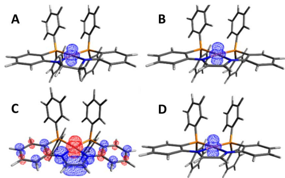
Fig. 8 (A) Spin density plot of 1 (isoval = 0.008). (B) Spin density plot of 2 (isoval = 0.04). (C) Spin density plot of 5^0_{OS} (isoval = 0.004). (D) Spin density plot of 6 (isoval = 0.008).
