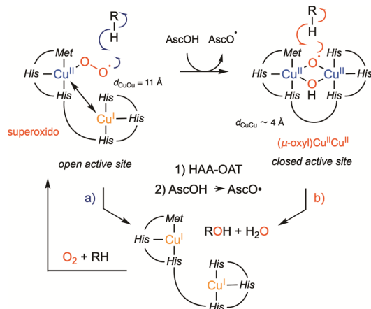
Scheme 2 Recently revisited mechanism for PHM and DβH showing the mechanisms involving an HAA by (a) \text{Cu}_M -superoxido intermediate in an open dicopper active site and (b) \mu -oxyl dicopper intermediate in closed dicopper active site. Abbreviation: AscOH for ascorbic acid.
