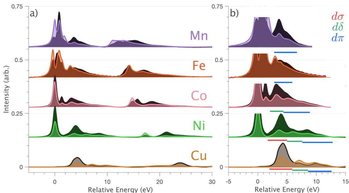
Fig. 4 (a) Single crystal L 2,3 -edge XAS of Li 2 (Li 1-x TM x )N, where TM = Mn, Fe, Co, Ni and Cu measured at 21 K. Normal incidence ( \vec{E} \perp c , \theta = 0^\circ ) spectra are shown in light colours and grazing incidence ( \theta = 70^\circ ) spectra are shown in dark colours. (b) The high energy side of the L 3 -edge region of the spectra is shown to emphasise charge-transfer satellites, labelled with an underline in red ( d\sigma ), green ( d\delta ) and blue ( d\pi ).
