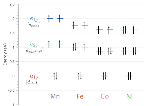
Fig. 5 Energy of 3d orbitals for Li 2 (Li 1-x TM x )N (where TM = Mn, Fe, Co and Ni) obtained via SA-CASSCF/NEVPT2 AILFT calculations.
