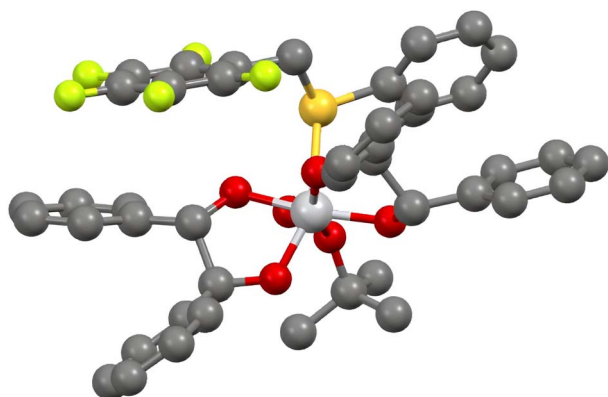
Fig. 1 Pro-( R ) titanium complex in the oxidation of pentafluorobenzyl phenyl sulfoxide. Hydrogen atoms are omitted for clarity. See ref. 27.
