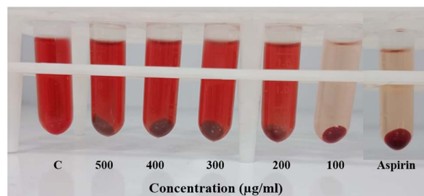
Fig. 13 Hypo-salinity induced hemolysis percentage inhibition. The x-axis of the bar graph shows the concentrations of BP-AgNPs and the lighter colored bar represents 500 \mu\text{g mL}^{-1} of aspirin. In pictorial illustration of hypo-salinity induced hemolysis inhibition, the symbol C represents the control with no inhibitor and aspirin was tested at a concentration of 500 \mu\text{g mL}^{-1} .
