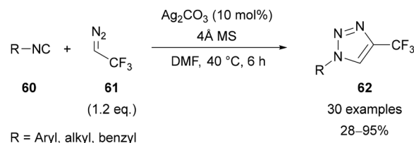
Scheme 21 Synthesis of 4-trifluoromethyl-triazoles from isocyanides and 2,2,2-trifluorodiazoethane.
