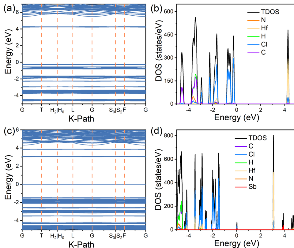
Fig. 4 DFT simulations. (a) electronic band structures and (b) density of states (DOS) of (TMA) 2 HfCl 6 ; (c) electronic band structures and (d) DOS of Sb 3+ -doped (TMA) 2 HfCl 6 .
