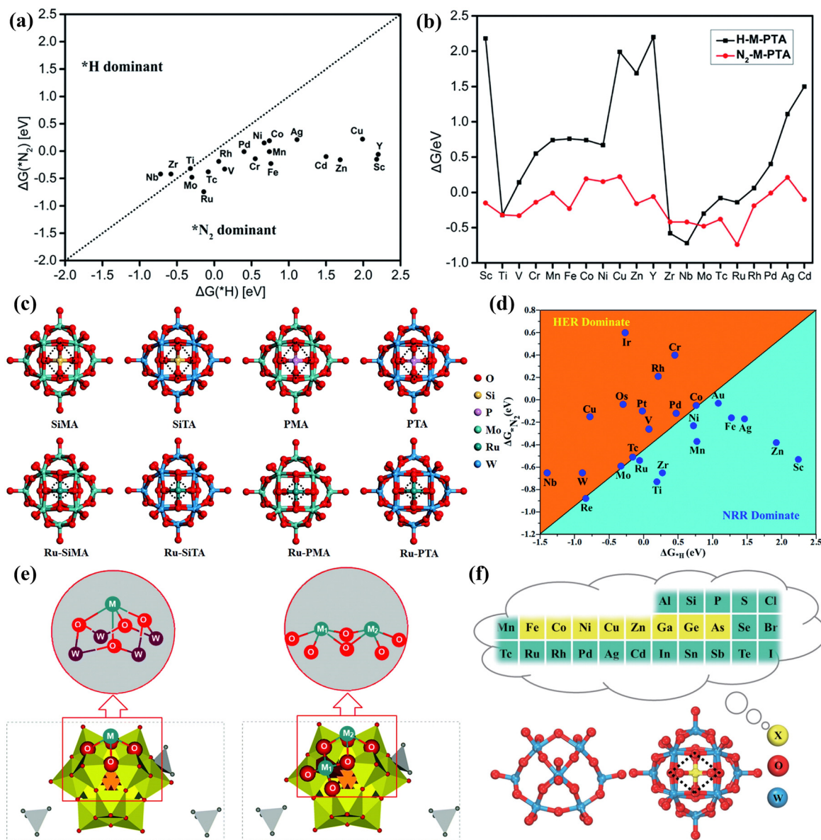
Fig. 17 (a) The calculated \Delta G(^*N_2) and \Delta G(^*H) on M-PTA. (b) The Gibbs free energy of *N_2 and *H adsorbed on M-PTA. 171 Copyright 2019, Royal Society of Chemistry (RSC). (c) Optimized structures of POM and Ru-POM. 172 Copyright 2020, Royal Society of Chemistry (RSC). (d) Calculated Gibbs free energies of N_2 and H_2 adsorbed on the M_1/PMA cluster. 173 Copyright 2022, Royal Society of Chemistry (RSC). (e) The structure of [N(CH_3)_4]^+_3[Ta^{II}_2/POM] (POM = [PW_{11}O_{39}]^{7-} ). 174 Copyright 2022, Royal Society of Chemistry (RSC). (f) Optimized structures of POM. 175 Copyright 2023, Springer, Tsinghua University Press 2022.
